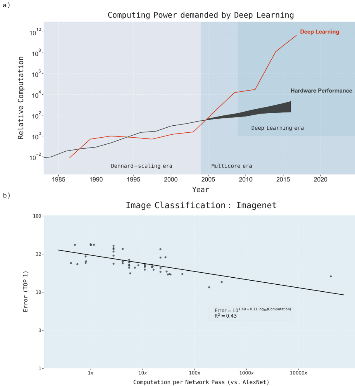
Figure 2: Computing power used in: (a) deep learning models of all types [5] (as compared with the growth in hardware performance from improving processors[23], as analyzed by [39] and [56]) 8 , (b) image classification models tested on the ImageNet benchmark (normalized to the 2012 AlexNet model [52]).
